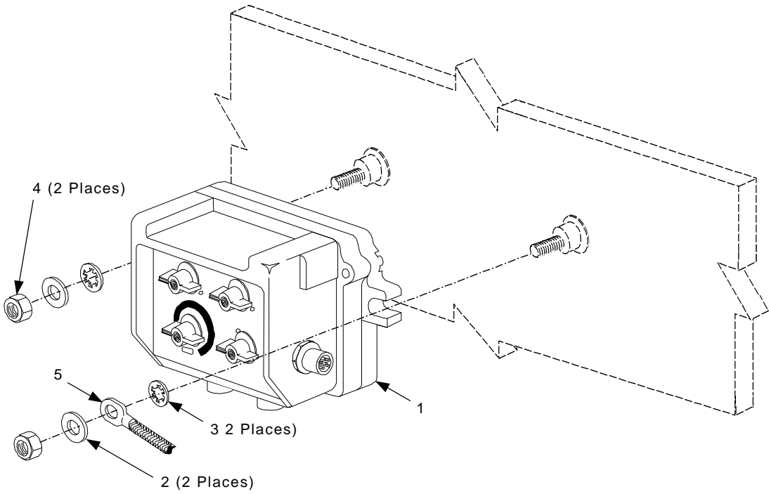
Figure 4-7. Gunner's FFCS Installation
