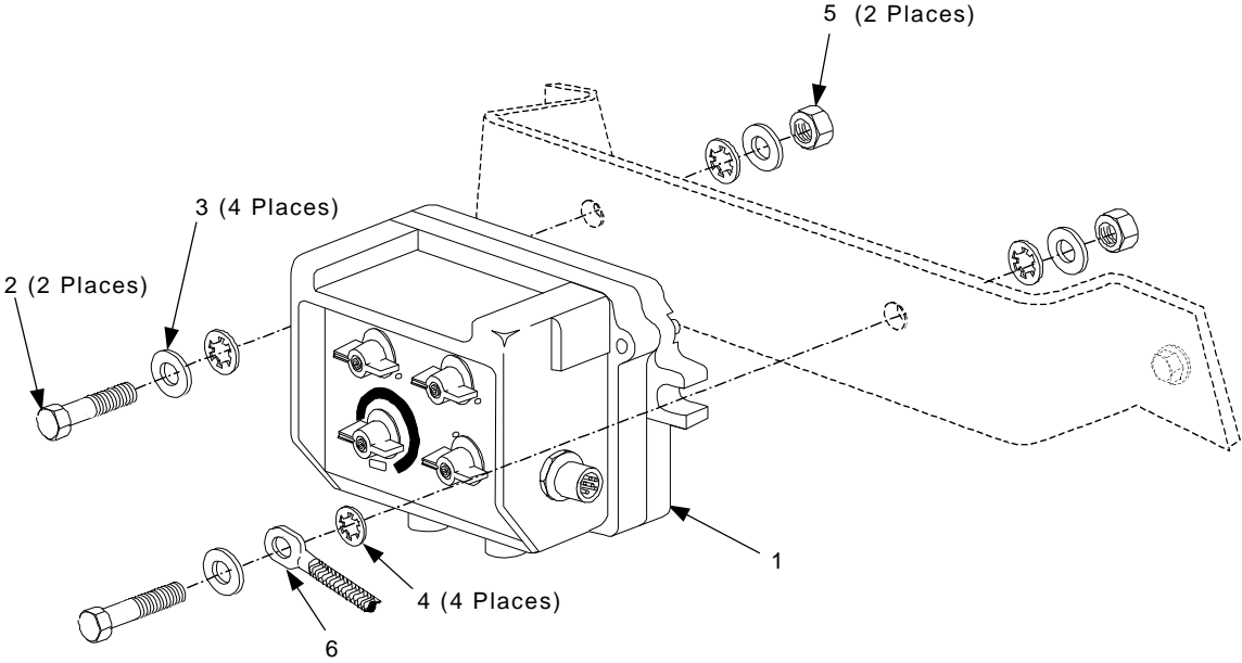
Figure 4-5. Driver's FFCS Installation
