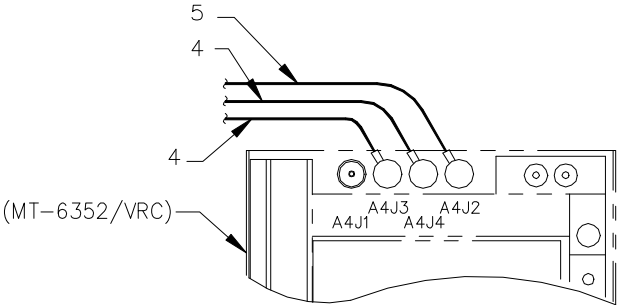
Partial View of Radio Mounting Tray
