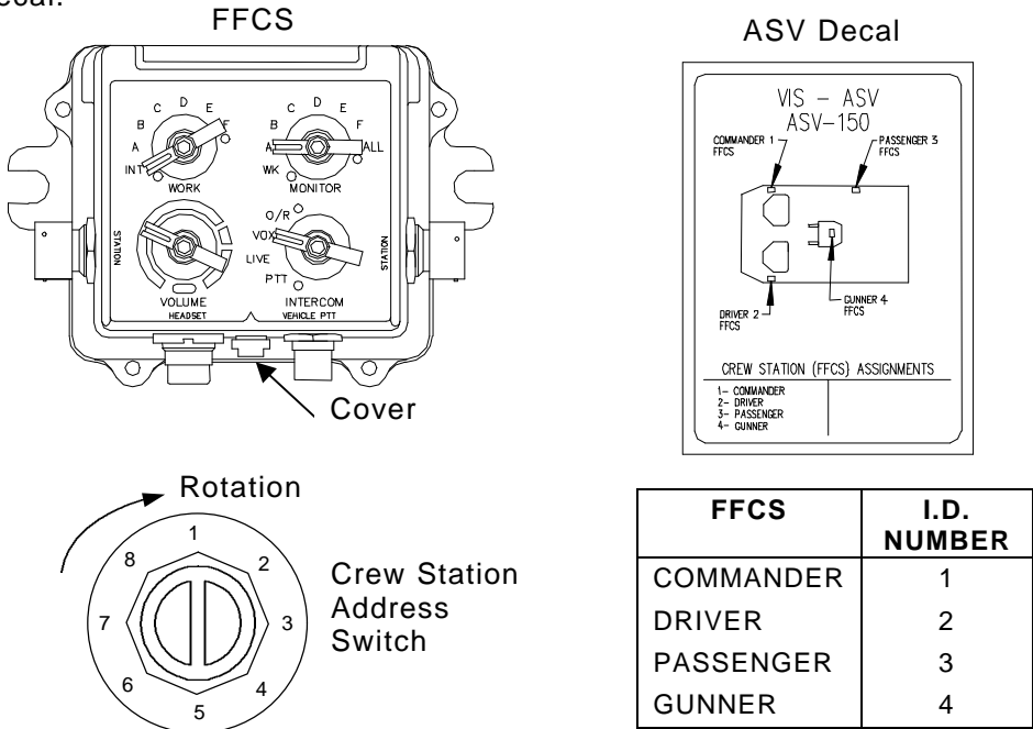
Figure 3-1. FFCS Crew Station Address Switch
