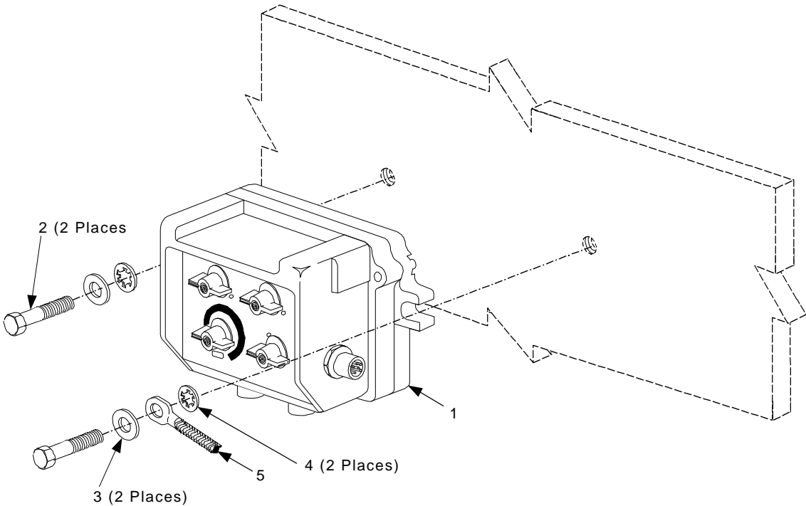
Figure 4-6. Passenger's FFCS Installation
